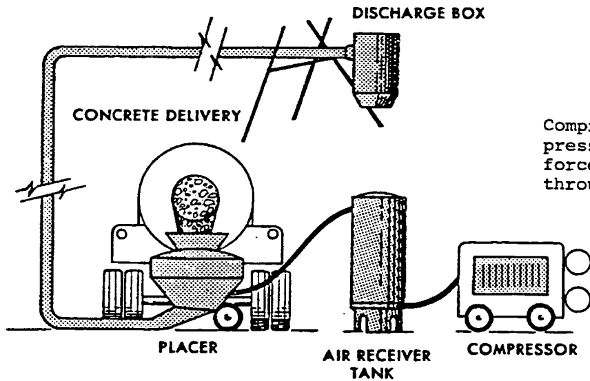
Figure 13: Pneumatic type concrete pump
